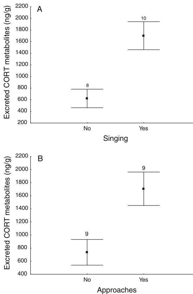
Fig. 2 Mean \pm SE CORT metabolites concentration of males that expressed singing behavior (a) or approximation (b) behavior when exposed to a playback of a conspecific male under their nestbox
