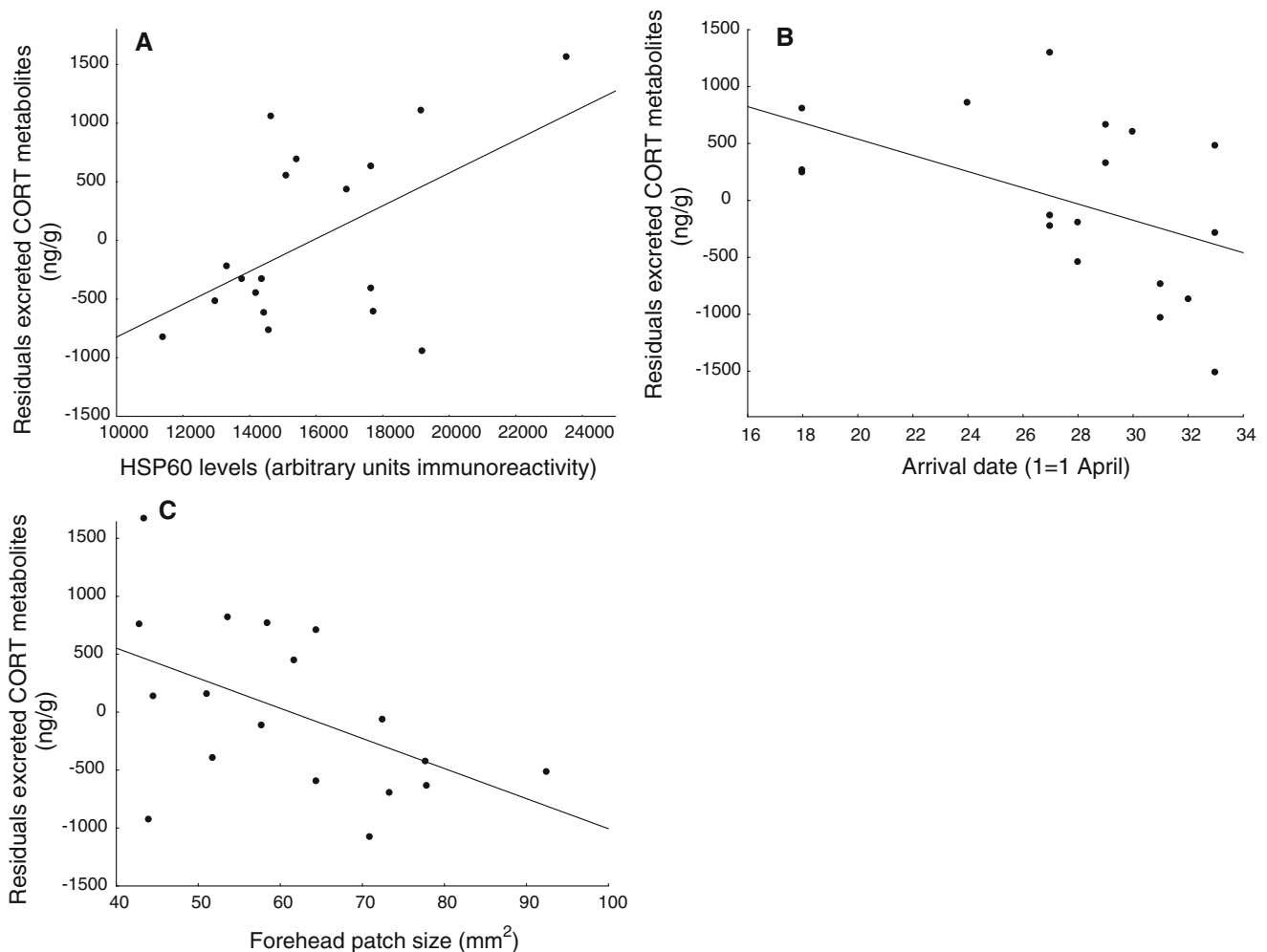
Fig. 1 a Association between HSP60 levels and the residuals of the regression of CORT metabolites on arrival date and forehead patch size. b Association between arrival date and the residuals of the
