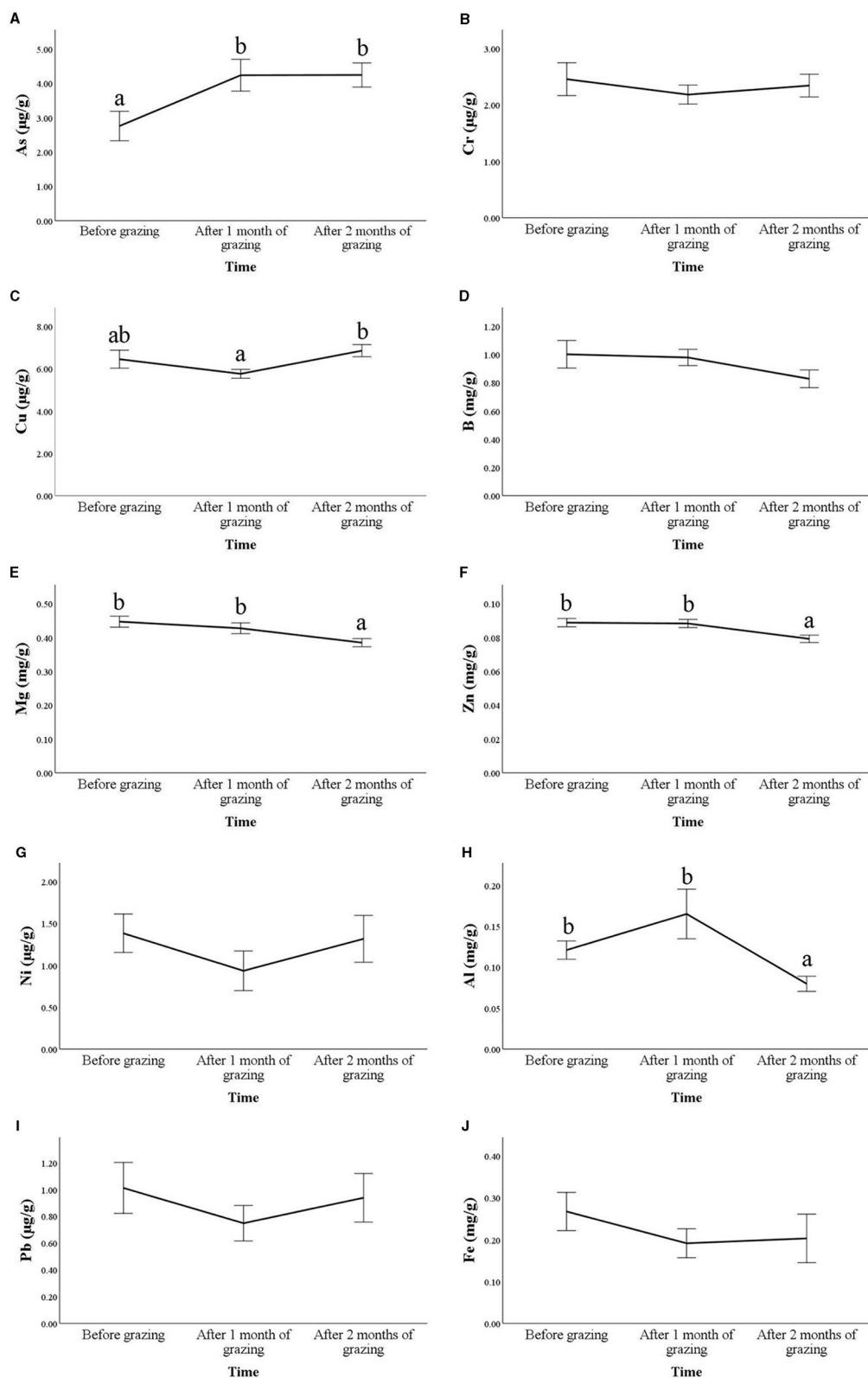
FIGURE 1 Hair concentrations of trace elements and heavy metals, expressed as \mu\text{g/g} or \text{mg/g} of hair, of Frisa goats during vertical transhumance. Hair samples were collected for 2 consecutive years ( n = 10 in 2021 and n = 17 in 2022), 1 day before vertical transhumance (before grazing) and 1 month and 2 months after vertical transhumance. For each molecule, time points that do not share the same letter are different for p < 0.05 . The time effect was not significant for molecules where no letters are present. The figures show the results for As (A), Cr (B), Cu (C), B (D), Mg (E), Zn (F), Ni (G), Al (H), Pb (I), and Fe (J). Values are means \pm standard errors (SE).
