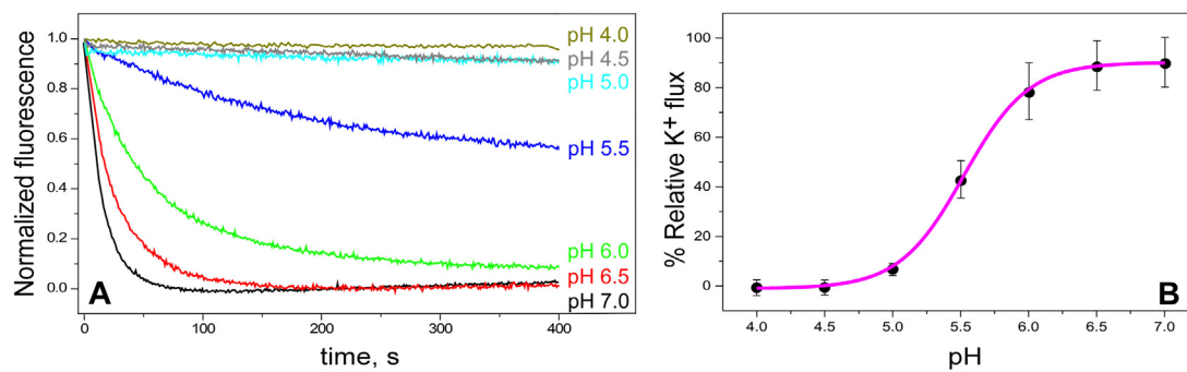
FIGURE 2 KirBac1.1 activity vs. pH. Panel (A), representative time-dependent quenching curves of ACMA fluorescence after addition of the protonophore CCCP (zero time), indicative of K^+ flux through the channel. The samples consist on KirBac1.1 reconstituted in asolectin liposomes (10 mM HEPES pH 7, KCl 100 mM intravesicular) at different extravesicular pHs (in 200 mM NMDG) (see Section 2). Panel (B) shows the relative K^+ flux for KirBac1.1 at different pHs, calculated as described in Materials and Methods (Equations 2, 3), from curves such as those shown in Panel (A). Several different batches of the purified channel protein were used to prepare the samples included in the panel. The results are the average flux ( n = 3 ) \pm S.D. The continuous line represents the fit of a Hill equation (Equation 4 in Section 2) to the data, from which pH_{0.5} is calculated.
