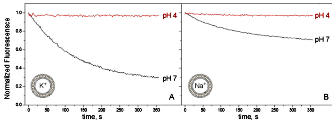
FIGURE 3 KirBac1.1 K^+ and Na^+ conduction at the macroscopic level. KirBac1.1 was reconstituted in asolectin liposomes (intravesicular buffers, 10 mM HEPES pH 7, KCl 100 mM, Panel (A); 10 mM HEPES pH 7, NaCl 100 mM, Panel (B)) and its activity was measured through the ACMA/CCCP assay. The same batch of purified protein was used to prepare all these samples to eliminate batch to batch variability and facilitate the comparison between the different experimental conditions. The extravesicular buffers are 10 mM HEPES pH 7, 200 mM NMDG ^+ (black) or 10 mM Succinic acid pH 4, 200 mM NMDG ^+ (red).
