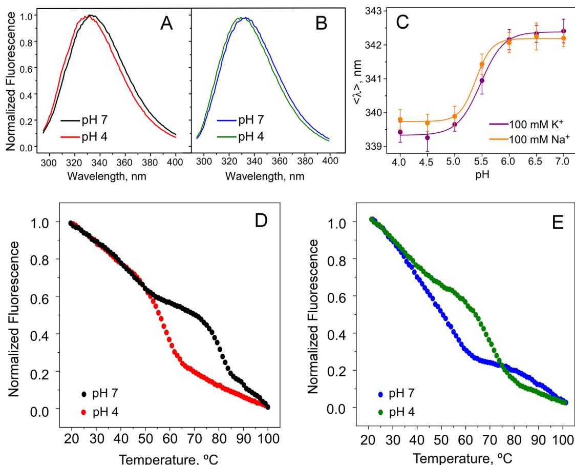
FIGURE 6 KirBac1.1 structure changes with pH. Normalized fluorescence emission spectra of KirBac1.1 at pH 7 and 4 (see Section 2), in buffers containing 100 mM KCl (A) or NaCl (B). The effect of pH on the intensity-weighted average emission wavelength ( \langle\lambda\rangle , Equation 6) in buffers containing 100 mM KCl or NaCl (C). The results are the average ( n = 3 ) \langle\lambda\rangle \pm S.D., measured at different pHs. The continuous lines represent the fit of a Hill equation (Equation 4 in Section 2) to the data, from which pH_{0.5} is calculated. The channel thermal denaturation assay at pH 7 and 4 in buffers containing 100 mM KCl (D) or NaCl (E). In all cases, purified KirBac1.1 solubilized in detergent (DDM) is used.
