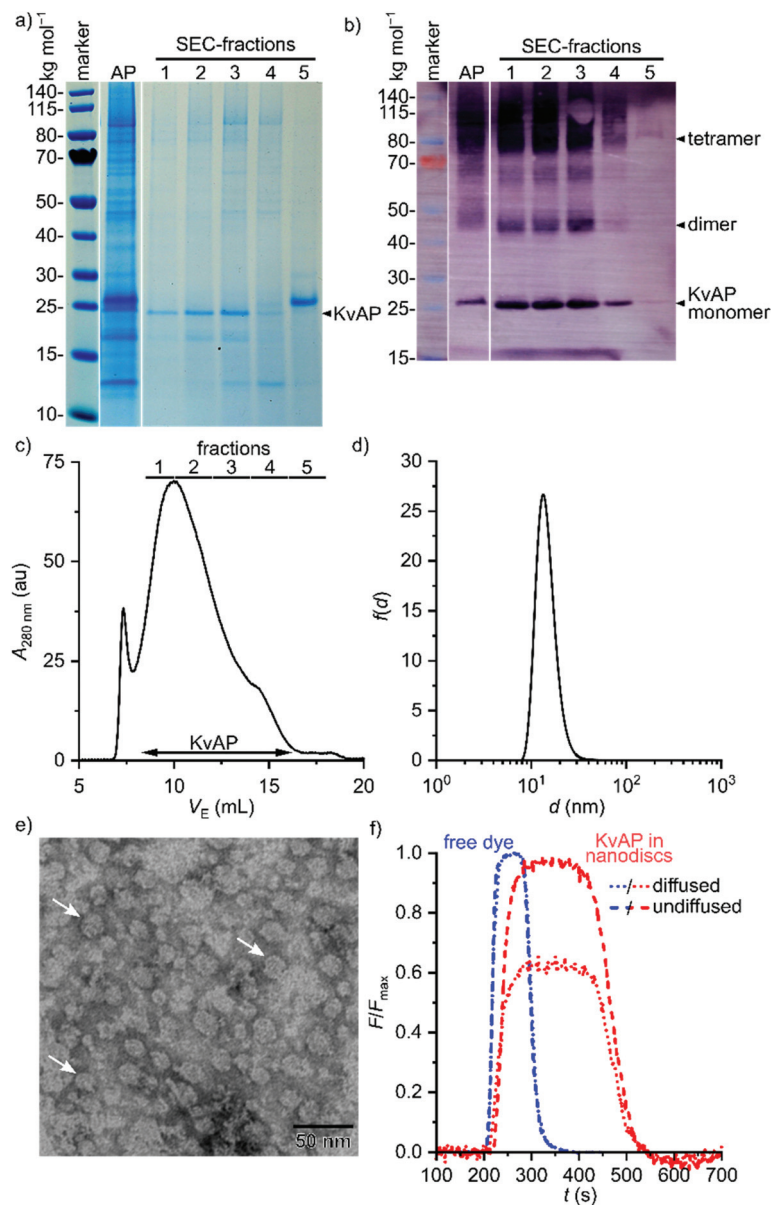
Fig. 7 Extraction and purification of the voltage-gated \text{K}^+ channel KvAP embedded in Glyco-DIBMA nanodiscs. (a and b) SDS-PAGE of KvAP extracted and purified with 5% (w/v) Glyco-DIBMA as visualized by (a) Coomassie stain and (b) western blot of two gels run with the same sample. Shown are samples after His 6 -tag affinity purification and concentration (AP) and after SEC as indicated in panel c. (c) Representative SEC elution profile of the concentrated sample (AP) shown in panels a and b on a Superose 6 Increase column. Shown is the absorption at 280 nm as a function of elution volume, V_E . (d) Number-weighted particle size distribution of Glyco-DIBMALPs harboring purified KvAP, as concentrated from SEC fraction 3 shown in panels a–c. (e) TEM image of KvAP-containing Glyco-DIBMALPs (same sample as shown in panel d). White arrows indicate nanodiscs in face-on views. (f) Normalized fluorescence emission intensity at \sim 520 nm of labeled KvAP (from SEC fraction 3) and unconjugated ATTO-488 maleimide after injection into a microfluidic laminar flow chamber and separation into two detection channels corresponding to diffused (dotted lines) and undiffused fluorophores (dashed lines).
