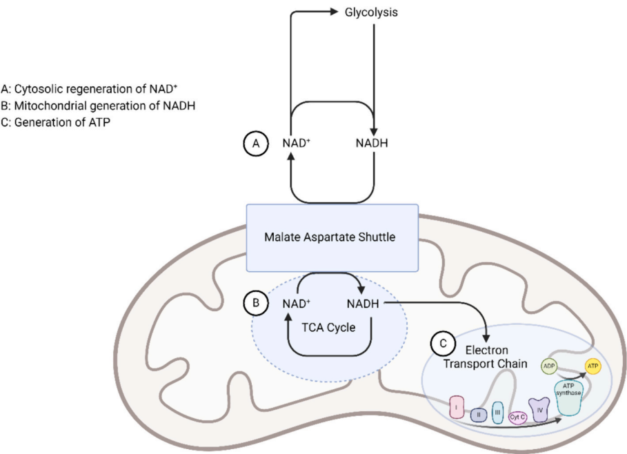
Fig. 2. Illustration showing how the malate aspartate shuttle links glycolysis, TCA cycle and electron transport chain. The malate aspartate shuttle (MAS) links glycolysis, the tricarboxylic acid (TCA) cycle and the electron transport chain (ETC). Because the inner mitochondrial membrane is impermeable for NADH, the MAS is required to shuttle electrons into the mitochondria. The MAS regenerates cytosolic NAD + enabling continuation of glycolysis (A) and generates mitochondrial NADH (B) which delivers its electrons to the ETC to ultimately generate ATP (C). Figure created with BioRender.com.
