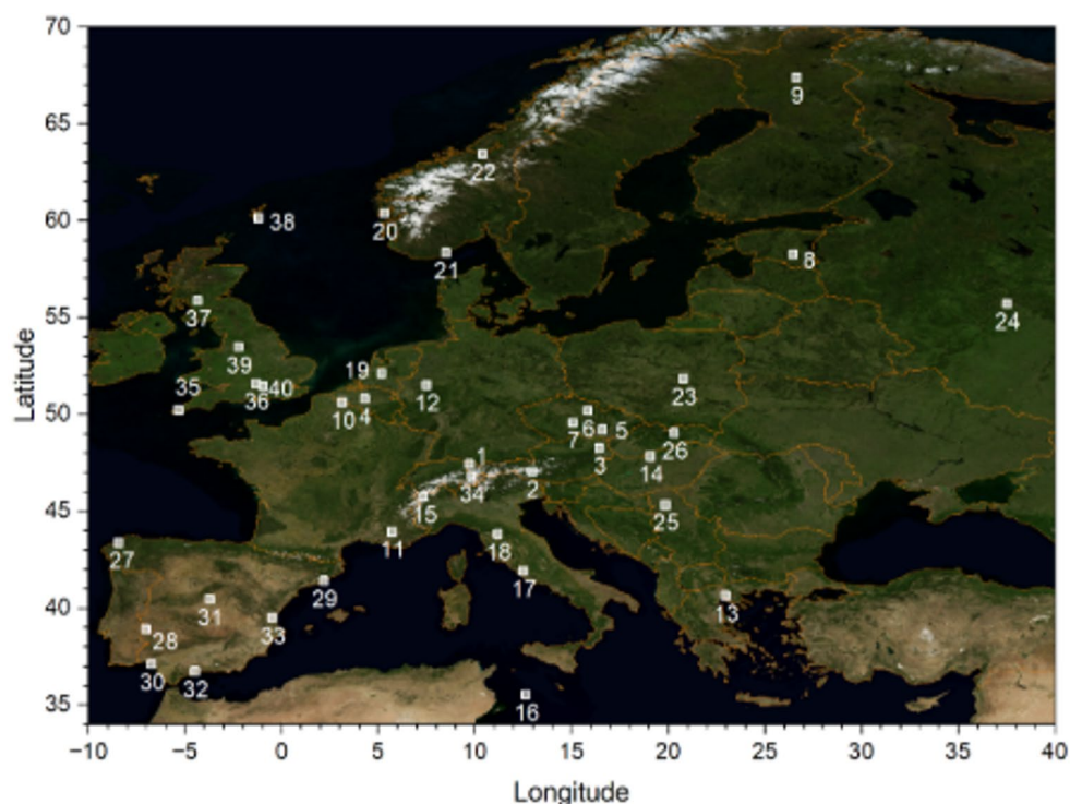
Fig. 1 Stations contributing data in this study on the Blue Marble Map, July 2004 from NASA Earth Observatory [47]
