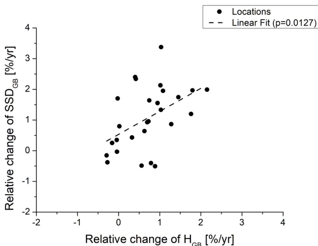
Fig. 5 Changes in annual mean of ground-based sunshine duration SSD_{GB} versus changes in annual mean of H_{GB}
