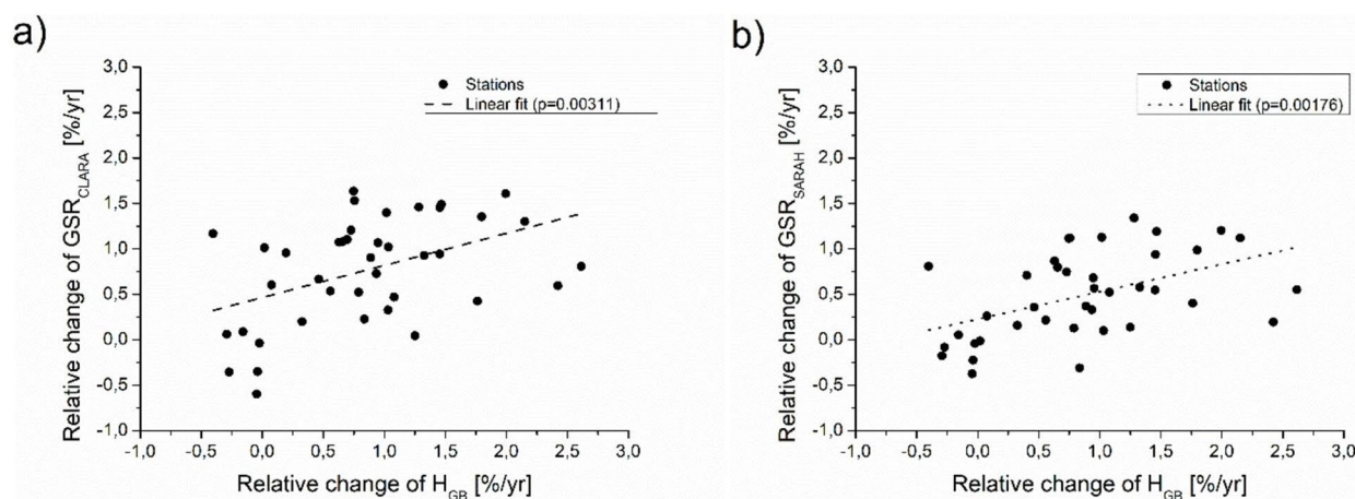
Fig. 7 Relative changes of annual means in ground-based UVR measurements ( H_{GB} ) compared to relative changes of annual means in global solar radiation gained (a) from CLARA ( GSR_{CLARA} ) and (b) from SARAH ( GSR_{SARAH} )
