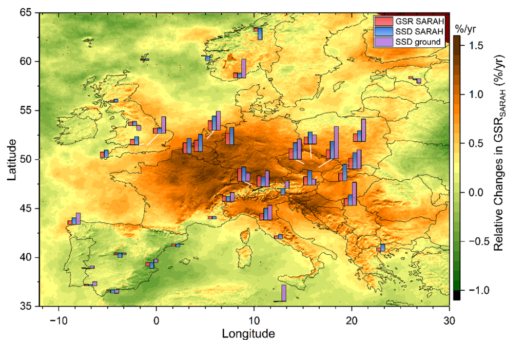
Fig. 6 Relative changes in sunshine duration measured at the ground (SSD ground, violet columns, if available), from space (SSD SARAH , blue columns) and changes in global solar radiation (GSR SARAH , red columns) for all locations underlain by the relative change in global solar radiation from SARAH
