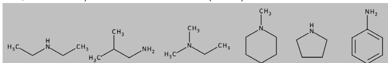
Abb. 7.7: Amine
