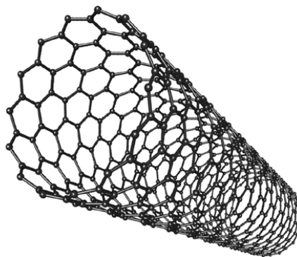
Abb. 3.18 b: Nanotube
